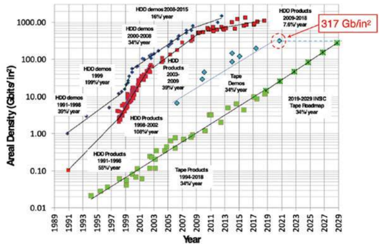
317 Gb/in 2 demonstrates the sustainability of the INSIC Tape Roadmap 34% CAGR in Areal Density for the next decade
