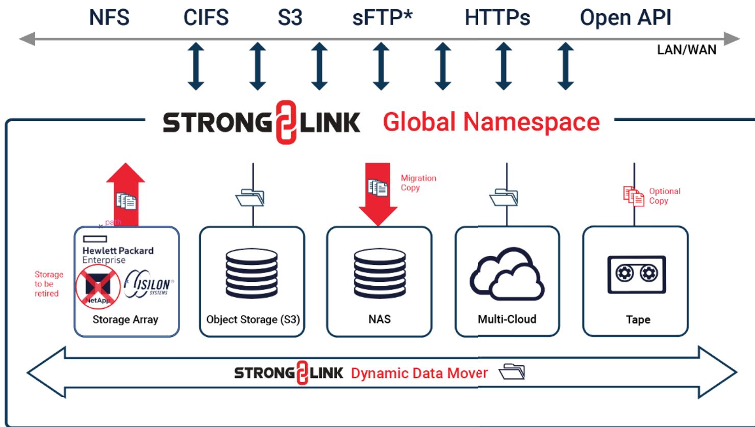
Figure 1. StrongLink ensures copies are migrated from the source storage to new target storage and verified
