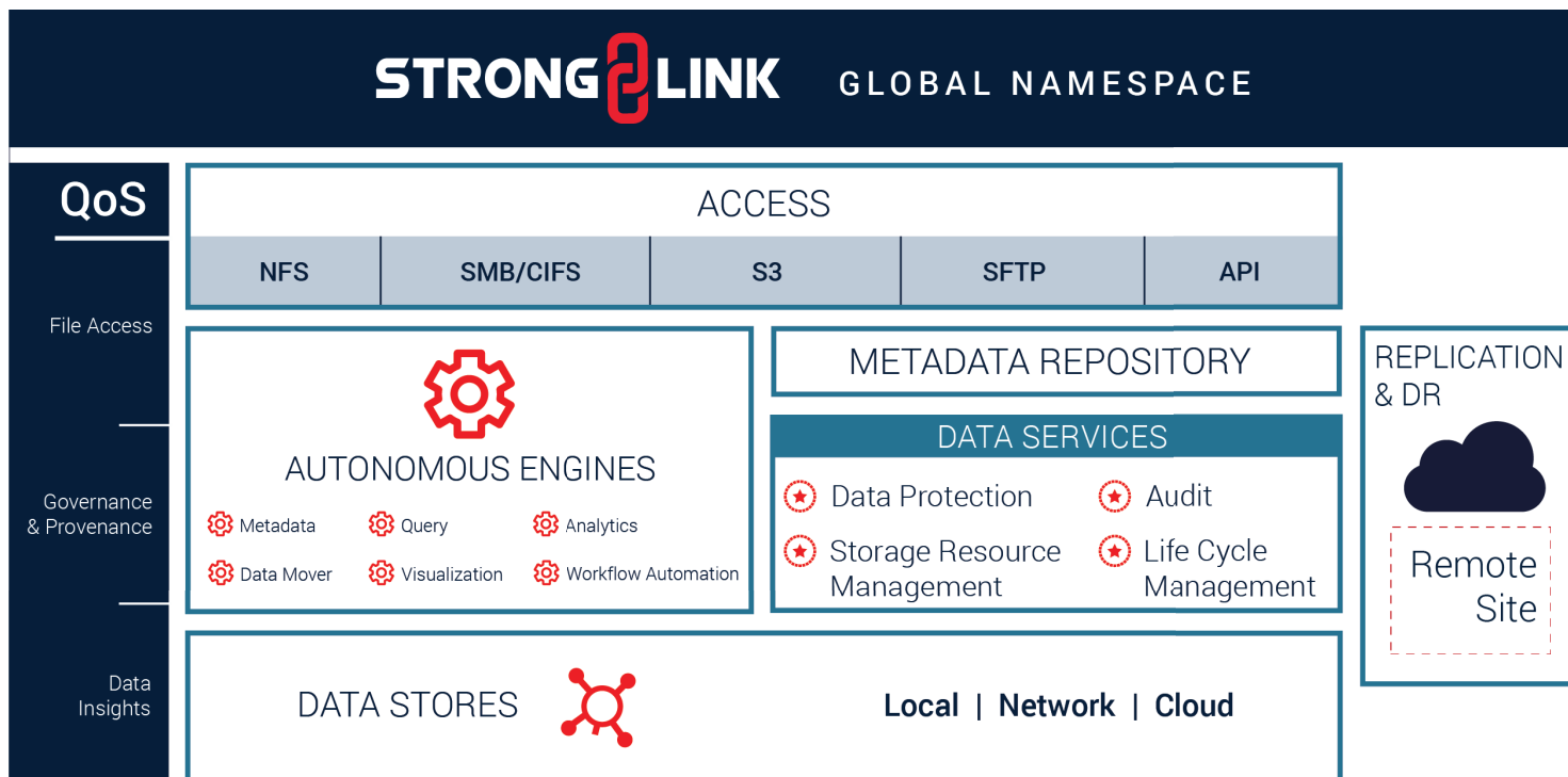
Figure 5. StrongLink architecture
